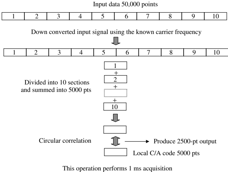
FIGURE 12.2 Folding 10 ms of data into 1 ms.
