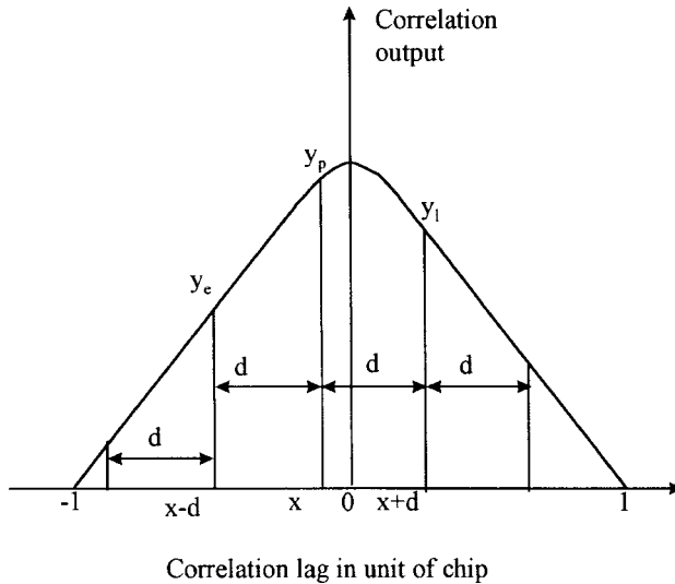
FIGURE 8.13 Correlation Output with Limited Bandwidth.
