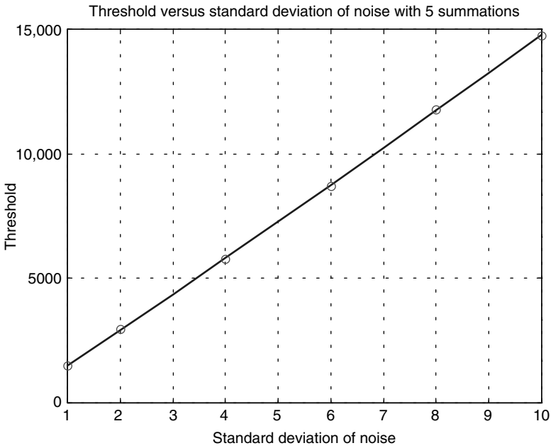
(b) 5 summations.
