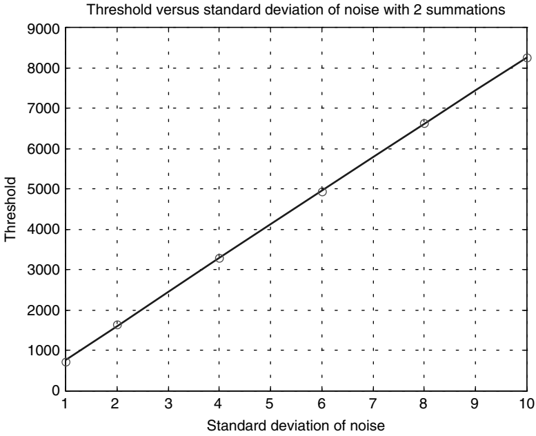
(a) 2 summations.
