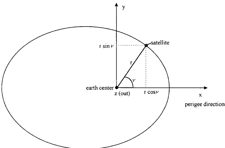
FIGURE 4.2 Orbit frame.
